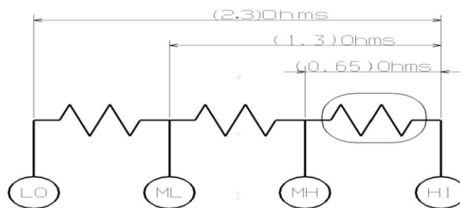
CIRCUIT OF DIAGRAM (at AMBIENT 25°C)
